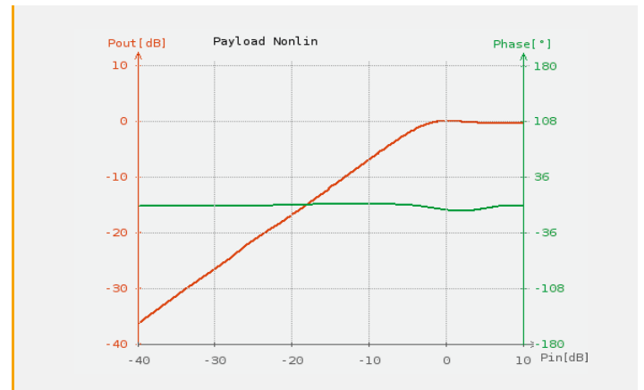
FIGURE 8: LTWTA CURVE: AM/AM AND PHASE VERSUS IBO DISTORTION
