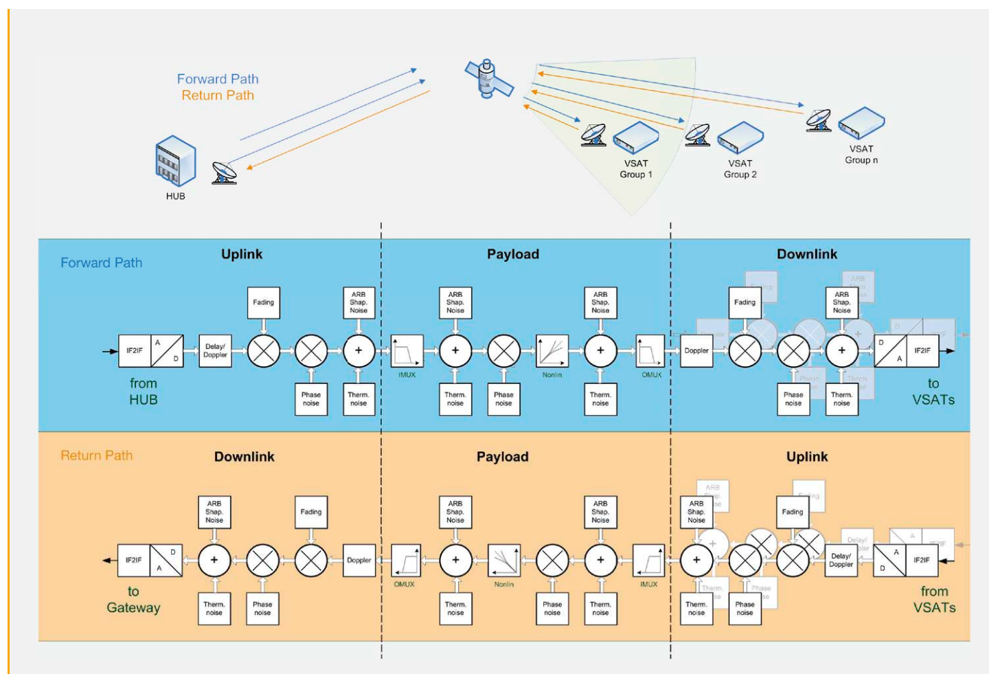
FIGURE 1: CHANNEL AND PAYLOAD MODELS OF IZT C6000
