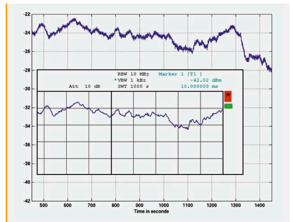
FIGURE 13: EXAMPLE OF A RAIN FADE SIMULATION
