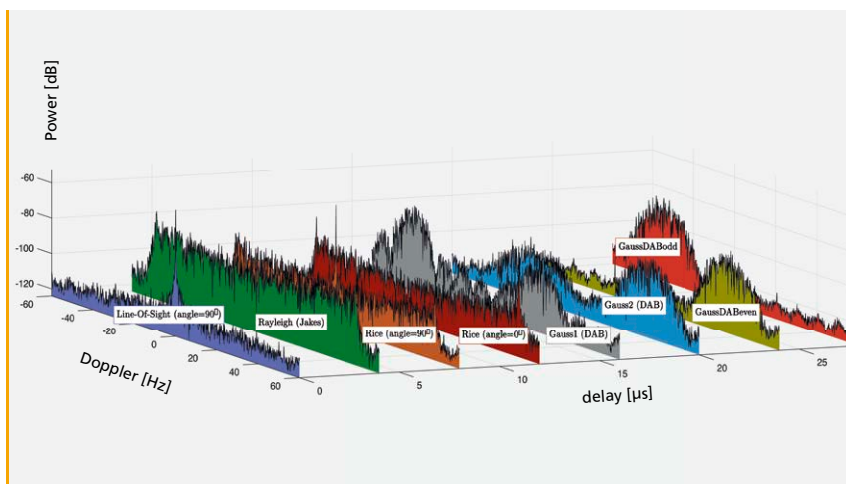
FIGURE 12: DOPPLER DELAY SPECTRUM
