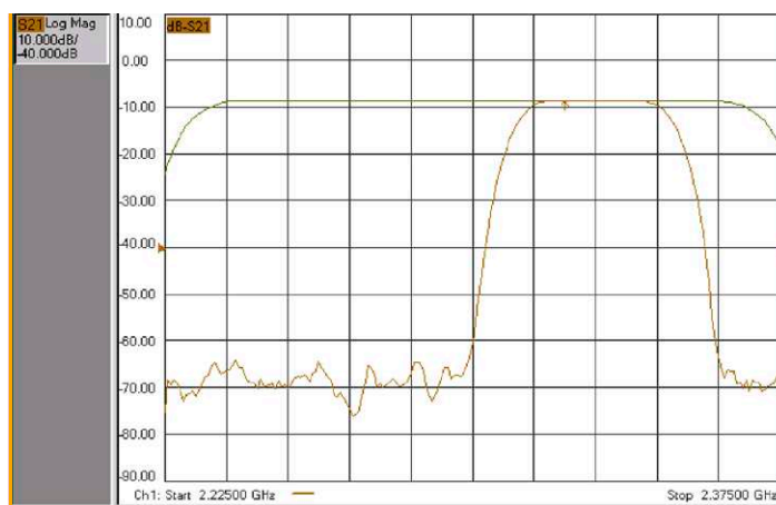
FIGURE 7: IMUX AND OMUX FILTERING
