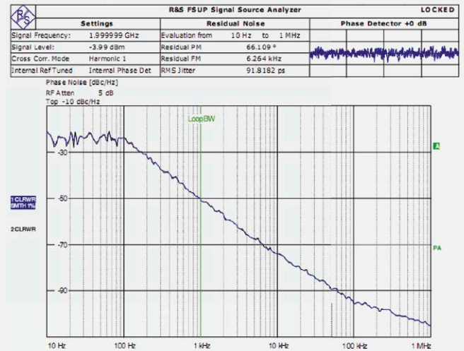
FIGURE 9: SIMULATED PHASE NOISE "DVB-S2 TYPICAL"
