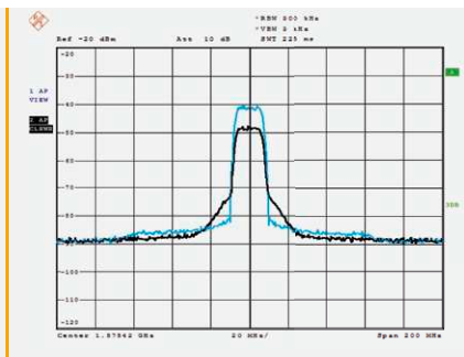
FIGURE 11: NONLINEARITY SIMULATION WITH A QAM SIGNAL
