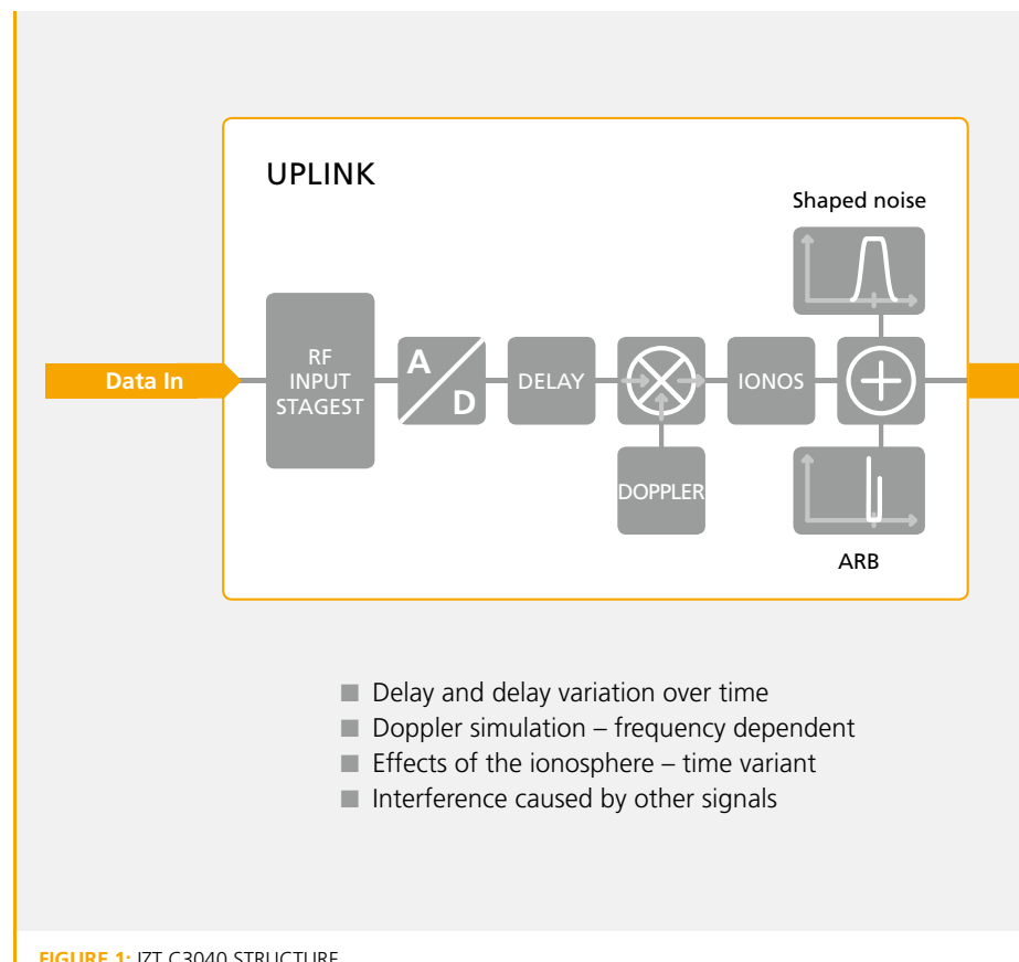
FIGURE 1: IZT C3040 STRUCTURE
