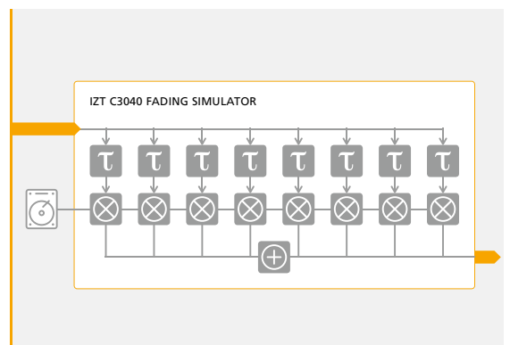
FIGURE 15: BLOCKDIAGRAM OF THE FADING SIMULATOR
