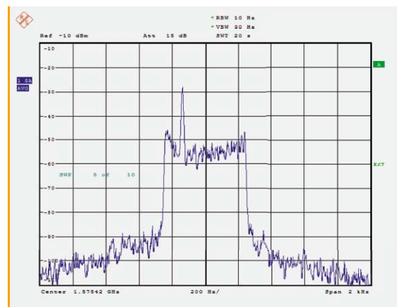
FIGURE 14: RICIAN FADING
