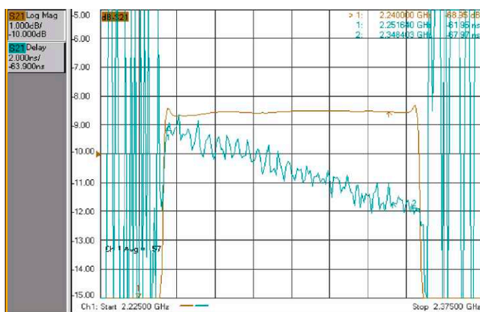
FIGURE 6: EMULATION OF THE IONOSPHERE WITH IZT C3040
