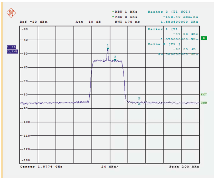
FIGURE 8: SIGNAL WITH INTERFERER
