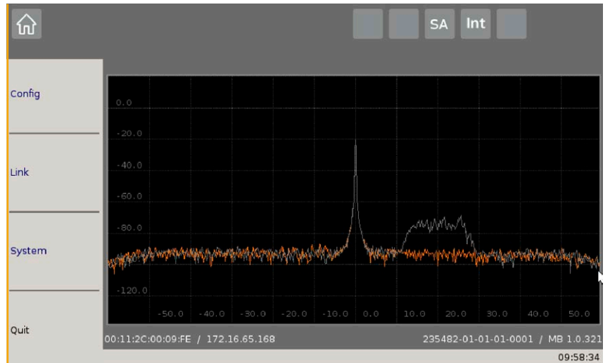
FIGURE 3: SPECTRUM DISPLAY
