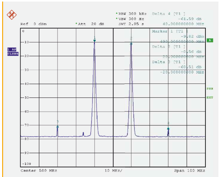
FIGURE 17: IZT C3040 THIRD ORDER INTERMODULATION PRODUCTS
