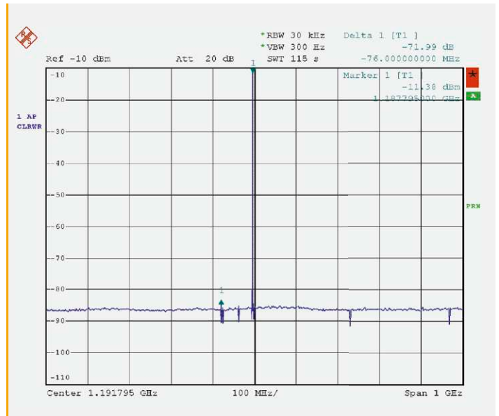
FIGURE 16: EXCELLENT SPURIOUS PERFORMANCE AND SIGNAL-TO-NOISE RATIO
