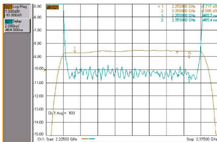
FIGURE 5: IZT C3040 GAIN AND GROUP DELAY FLATNESS
