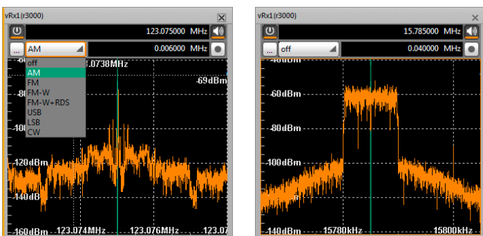
FIGURE 4+5: SPECTRUM, DEMODULATION AND RECORDING OF DETECTED SIGNALS
