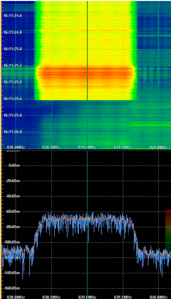
FIGURE 3: SUB-BAND MONITORING WITH SPECTRUM & SPECTROGRAM DISPLAY
