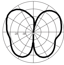
F = 400 MHz
