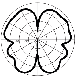
F = 1000 MHz
