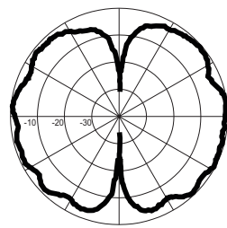
F = 2000 MHz
